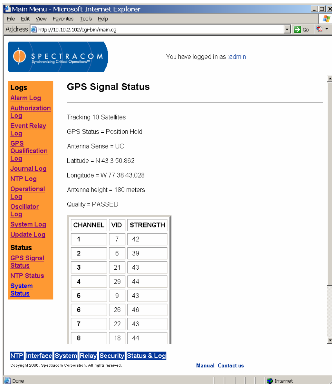
Figure 3-105: GPS Signal Status Screen
