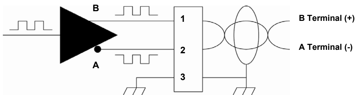
Figure 2-7: RS-485 Output
